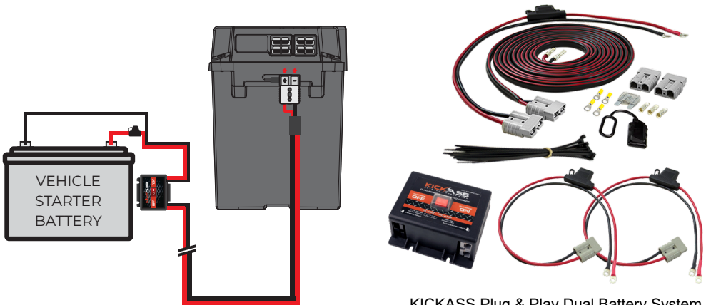
KICKASS Plug & Play Dual Battery System Wiring Kit & Dual Sensing VSR SKU: KADABE K8MMV SR2AND
